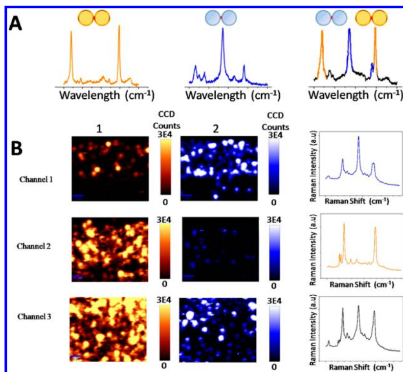
Figure 7. Example of SERS spectra. (A) SERS particles have unique spectra, which allow for multiplex detection. Here two sets of SERS reporter labels are shown with their unique spectra and then together, showing multiplex detection. (B) Nanoyeast–scFv affinity reagents were used for duplex detection of two different types of pathogen antigens in a three-channel microfluidic device. False-color images of SERS reporter particles binding to nanoyeast immobilized antigens, and their corresponding average SERS spectra are shown. Channels 1 and 2 each were coated with nanoyeast–scFv that were each specific toward one type of antigen. Channel 3 contained both types of nanoyeast–scFv, allowing for simultaneous duplex detection. Adapted with permission from ref 27. Copyright 2014 American Chemical Society.
