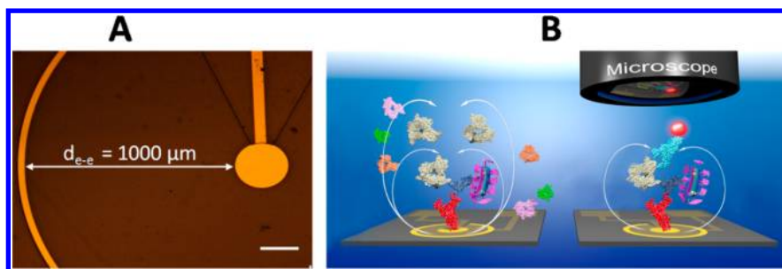
Figure 8. Schematic representation of the mechanism of ac-EHD induced surface shear forces for rapid capture and detection of antigen using nanoyeast–scFv as protein capture agents. (A) Optical image of the asymmetric electrode pair containing an inner circular small electrode and a large outer ring electrode with an edge to edge distance of 1000\ \mu\text{m} between the electrodes. The diameters of the inner electrode and the width of the outer ring electrode were 250 and 30\ \mu\text{m} , respectively. Scale bar = 200\ \mu\text{m} . (B) Schematic representation of the mechanism of ac-EHD induced surface shear forces for rapid capture and detection of a pathogenic antigen (not drawn to scale). A confocal microscope visualized detection antibody conjugated with quantum dots. Figure reproduced with permission from ref 29. Copyright 2015 American Chemical Society.
