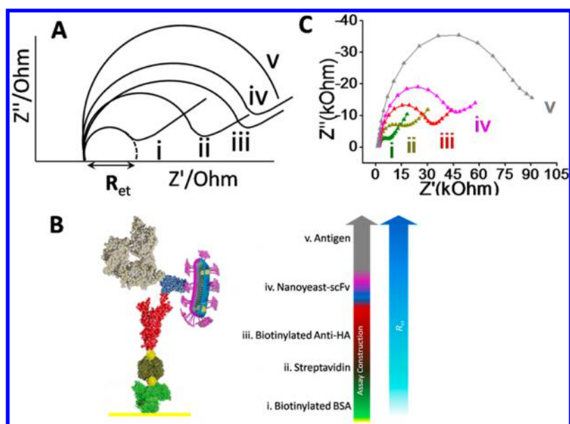
Figure 6. (A) Example of a Nyquist plot, which plots the real ( Z' ) and imaginary ( Z'' ) components of impedance measurements. As biomolecules at each step of an immunoassay are immobilized onto the biosensor layer on a conducting or semiconducting electrode, an increase in R_{et} is observed at each immobilization step. Here, we have an example of five different steps of an immunoassay being immobilized onto an electrode, which corresponds to a R_{et} increase at each step of i–v. (B) Construction of a nanoyeast–scFv biosensor, layer by layer, which causes the impedance to increase at each layer respectively as shown in the Nyquist plot in panel C. Sensor constructed on gold substrate. Panel B reprinted with permission from ref 26. Copyright 2014 Elsevier. Panel C adapted with permission from ref 25. Copyright 2013 The Royal Society of Chemistry.
